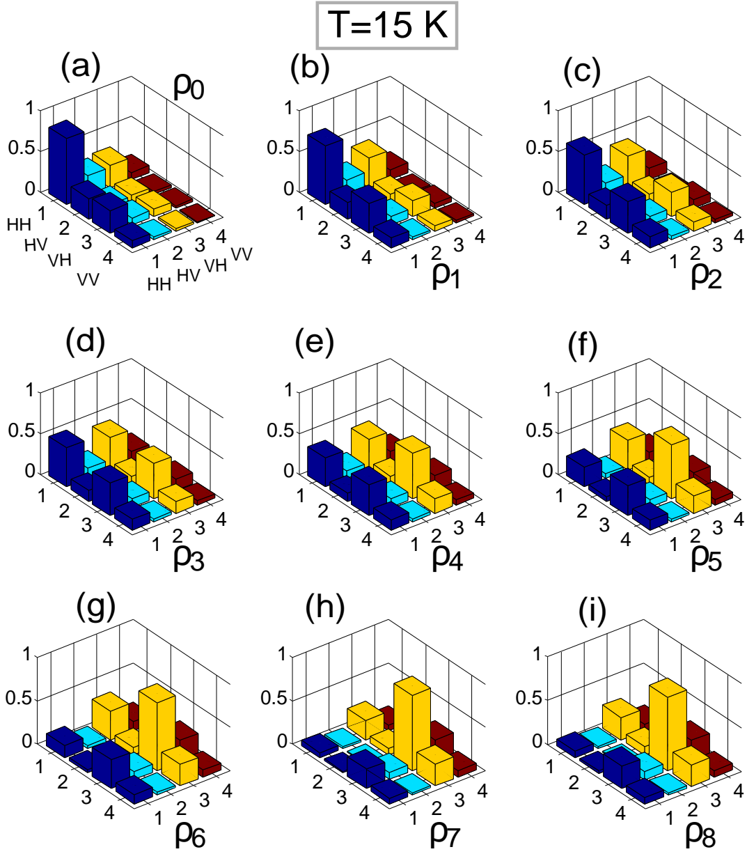
Figure 4.10: The density matrices reconstructed from tomography measurements at 15 K as a function of magnetic field. The density matrix (a) \rho_o corresponds to zero magnetic field whereas (b)–(i) are the density matrices for magnetic field range (1–3 A) with a step size of 0.25 A. The nominally generated input state is \rho_o = |HH\rangle\langle HH| .
