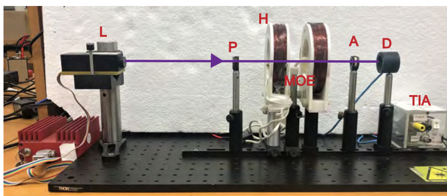
Figure 1.11: Experimental arrangement of the Faraday setup. The light exiting the source passes through the optical element before hitting the photodetector. Where L =laser, P =polarizer, H = Helmholtz coils, MOE = magneto-optical element, A = analyzer, TIA = trans-impedance amplifier and D = photodetector
