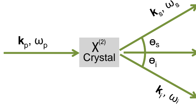
Figure 4.4: An illustration of spontaneous parametric downconversion of light where \hbar times the (\mathbf{k}_j, \omega_j) denotes the momentum and energy of the incoming and outgoing light whereas \theta_j signifies angle between the pump beam and outgoing photon beam. The subscripts p , s and i are attributed to the pump, signal and idler and \chi^{(2)} presents the non-linear electric susceptibility.
