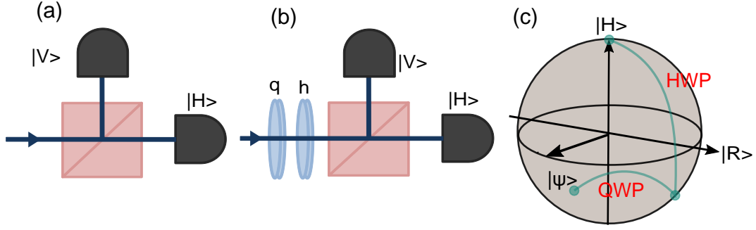
Figure 4.2: The projective measurement is performed along (a) \{|H\rangle, |V\rangle\} . (b) Measurement along \{|R\rangle, |L\rangle\} and \{|D\rangle, |A\rangle\} basis are realized by transforming the state into \{|H\rangle, |V\rangle\} basis using different setting ( q , h ) of quarter- and half wave-plates whereas (c) depicts the action of QWP and HWP on an arbitrary state in the Bloch sphere.
