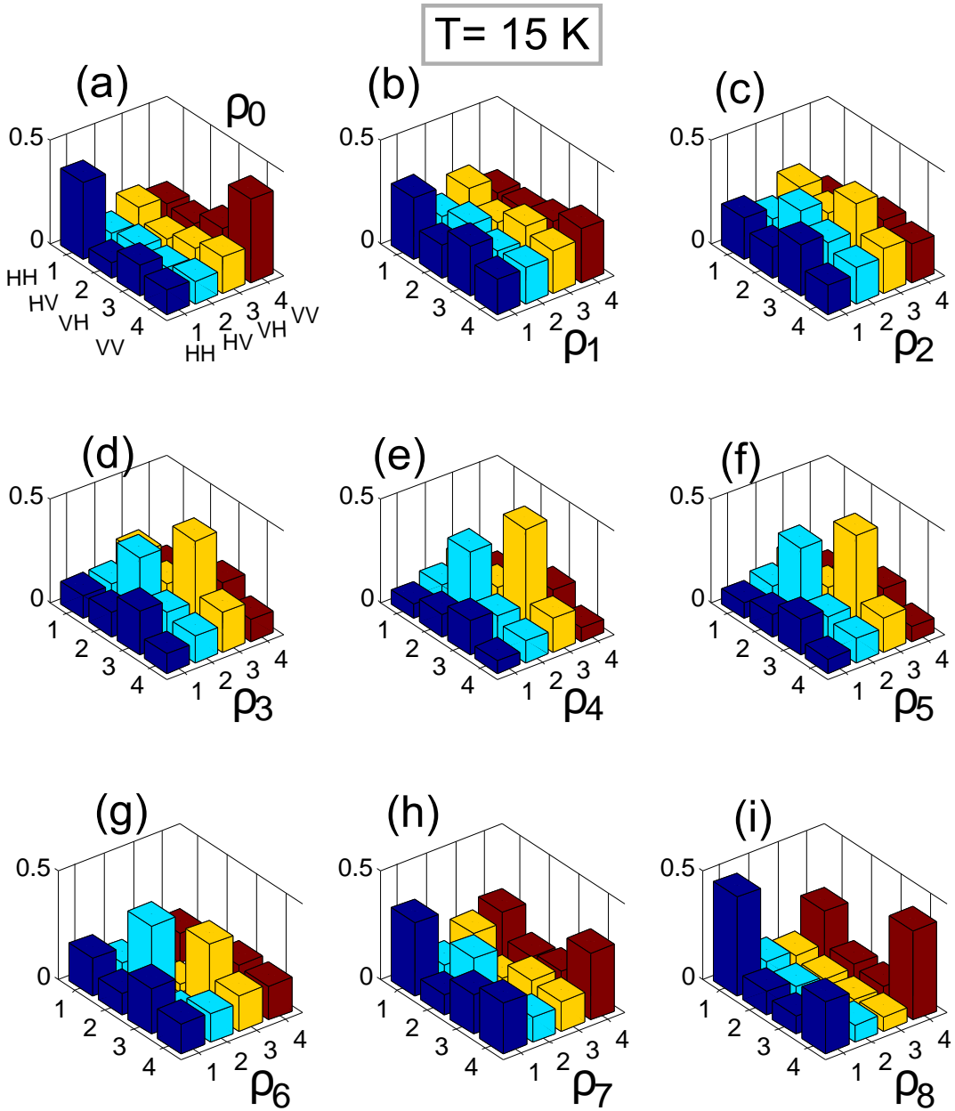
Figure 4.12: 3D plots of Bell's state |\phi^+\rangle at T = 015 K where (a) \rho_0 corresponds to zero magnetic field whereas for (b)–(i), the current through the EM coils is varied from 1–4.5 A with a step size of 0.5 A.
