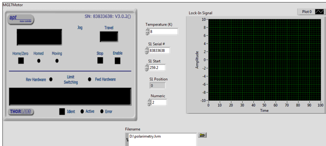
Figure A.5: Front panel of the Stokes polarimetry labview program. The graphical VI displays the output from the lockin channel whereas MG17Motor control shows the angular position of quarter waveplate which is being rotated in a step size of 5^\circ .
